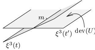
FIGURE 5. \text{dev}(U) .
