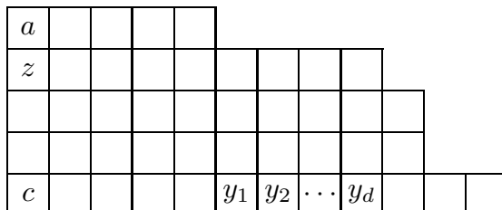
Fig. 2.1. Hook length and t -compact set
