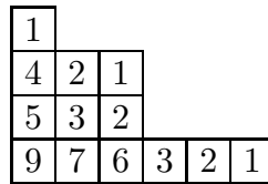
Fig. 1.2. Hook lengths
