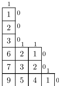
Fig. 2.1. Partition and (0,1)-sequence
