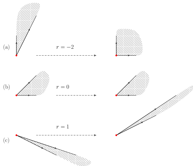
FIGURE 1. Normalization of various polygons when J has a global minimum. The red point corresponds to the image of the value (J_{\pm}, H_{-}) . The integer r indicates that a global transformation T^r was applied to the polygon in order to normalize it.
