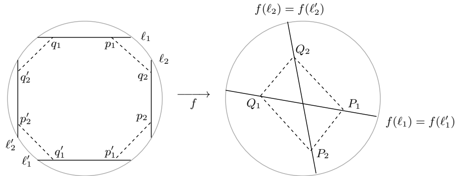
Figure 2: An illustration of the proof of Proposition 5.2 when S is a one-holed torus. The boundary of the lifted convex core \tilde{\Omega} \subset \mathbb{H}^2 is dashed. We set p'_i := j(\gamma_i) \cdot p_i and q'_i := j(\gamma_i) \cdot q_i , as well as P_i := f(p_i) = f(p'_i) and Q_i := f(q_i) = f(q'_i) .
