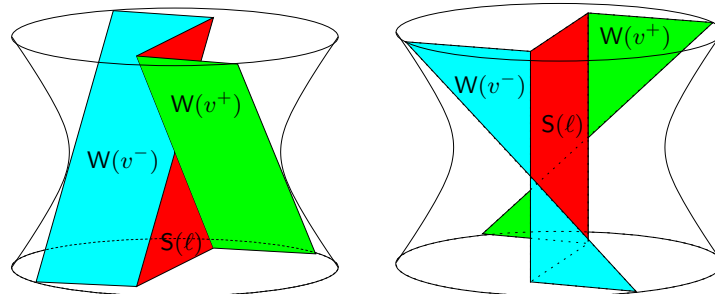
Figure 1: The left AdS crooked plane C(\ell) , seen in two different affine charts of \mathbb{P}^3(\mathbb{R}) \supset \text{AdS}^3 . The stem S(\ell) is a bigon whose closure in \mathbb{P}^3(\mathbb{R}) meets the boundary of \text{AdS}^3 in two points, tangentially. On the left, these two points are at infinity; on the right, the center of the stem is at infinity. Each wing W(v^+) or W(v^-) is itself a bigon, bounded by a line contained in the boundary of \text{AdS}^3 and a lightlike line of the stem S(\ell) .
