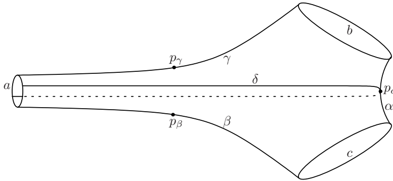
FIGURE 3. A thrice punctured sphere with a short loop.
