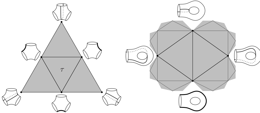
FIGURE 2. The arc complexes \overline{\mathcal{X}} of the two small surfaces.
