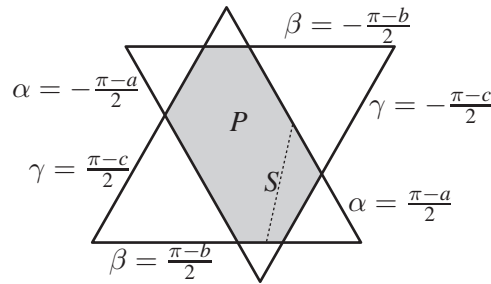
Figure 2: The hexagon P of solutions (\alpha, \beta, \gamma) to (2), and the segment S of spun angle structures. At most one pair of opposite sides of P can be reduced to points, because a, b, c < \pi .
