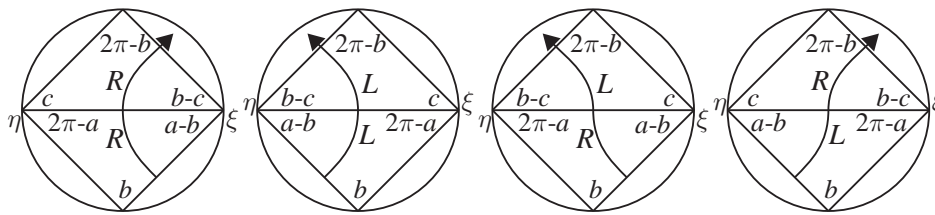
Figure 7: The Farey triangles T_{i-1} (lower) and T_i (upper), with corner labels.
