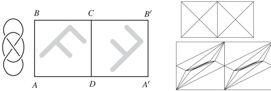
Figure 11: Left: the (chiral) Whitehead link m129. Middle: cusp view of m129 from the common tip of the square-based pyramids Q and Q' , i.e. from the cusp that will be filled. The F -shaped symbol drawn on the bases of Q and Q' shows their identification. Right: view of the canonical decomposition from the other cusp of m129, before (top) and after (bottom) a Dehn filling with (k, l) = (11, 8) . In the top panel, the centers of the two squares project to the cusp that will be filled. In the bottom panel, we see that the tetrahedra in the decomposition of the filling become very close to flat, very quickly.
