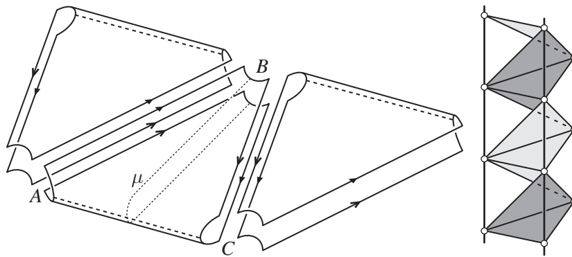
Figure 3: Left: a punctured torus (shown as 3 folded copies of a fundamental domain; arrows are identified) wraps around an ideal Möbius band. The meridian arc \mu , of slope m , becomes homotopically trivial. The dotted folding edge AC has slope m' . Right: part of the universal cover of the same Möbius band (shaded) and the tetrahedron \Delta_{N-1} glued to it.
